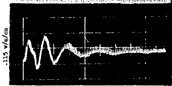
Fig. 3.101 Broadband pulse Shot No. 8 3400 km from ground zero
